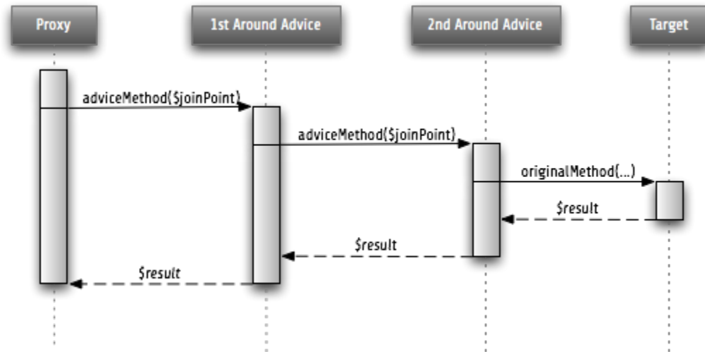
Fig. 26: Control flow of an advice chain
