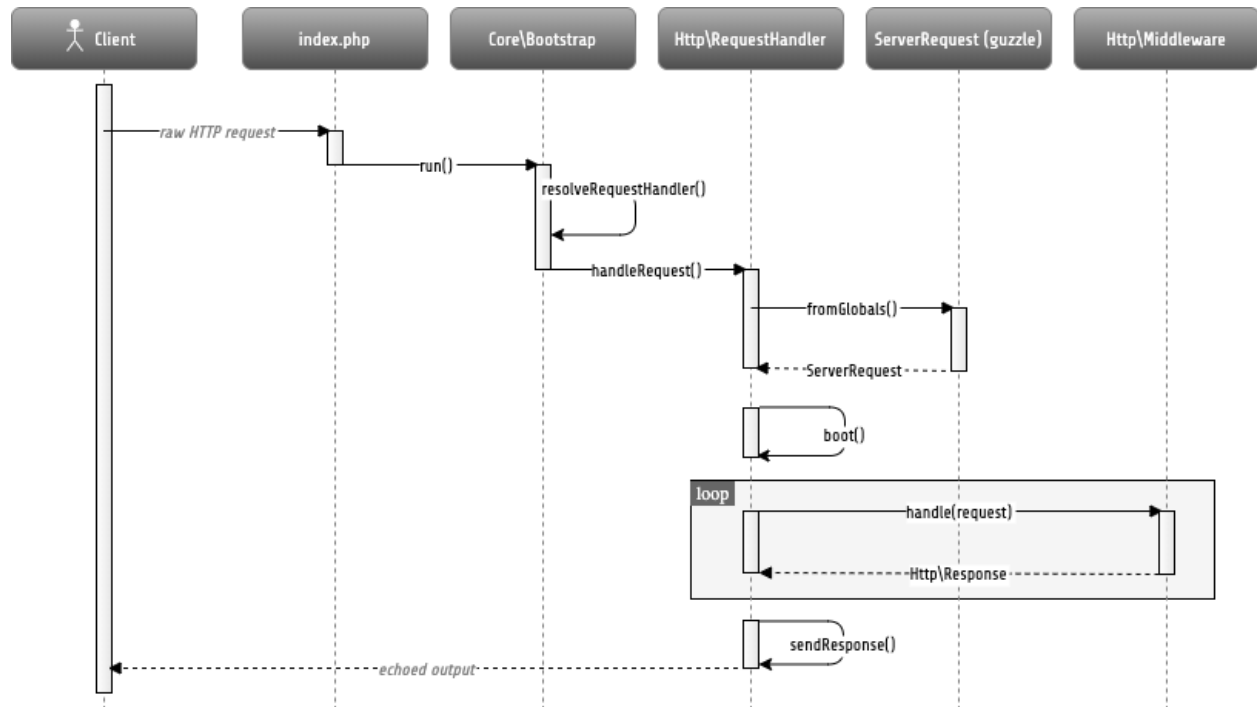
Fig. 25: Simplified application flow
